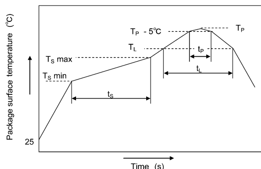
Fig. 10.2.1 Temperature Profile for Lead(Pb)-free Soldering (example) Table 10.2.1 Temperature Profile for Lead(Pb)-free Soldering (example)
