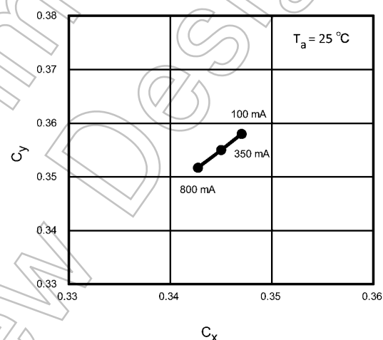
Fig. 8.4 Chromaticity - I_F
